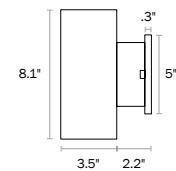
CORE 3 DIRECT/INDIRECT SCONCE
