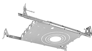
New Construction Kit W/ Hanger Bar [For Trim] [ICON-SR-2-4-NCH]
