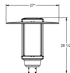
Slide Post Top Mount
