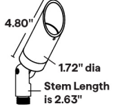
45 Degree Snoot (45D)
