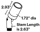
Flush Snoot (FL)
